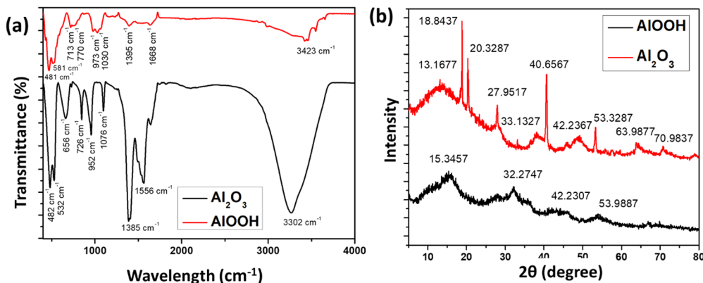
Fig. 2 FTIR (a) of \text{Al}_2\text{O}_3 (black) and ALOOH (red). XRD (b) of \text{Al}_2\text{O}_3 (red) and ALOOH (black).
