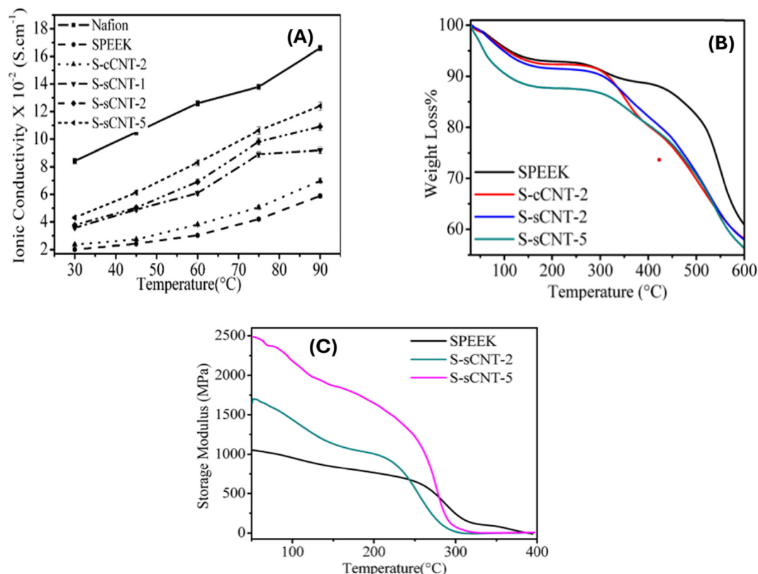
Fig. 15 (A) Proton conductivity vs. temperature, (B) TGA thermographs and (C) DMA of SPEEK, S-sCNT-2, and S-sCNT-5 membranes. 90
