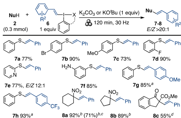
Scheme 3 Mechanochemical vinylation scope. Products 7 formed with VBX 6a–6c and \text{K}_2\text{CO}_3 , products 8 formed with salt 6d and \text{KO}^t\text{Bu} . a THF as LAG, 135 min; b 10 min; c 3.0 mmol scale; d 30 min.
