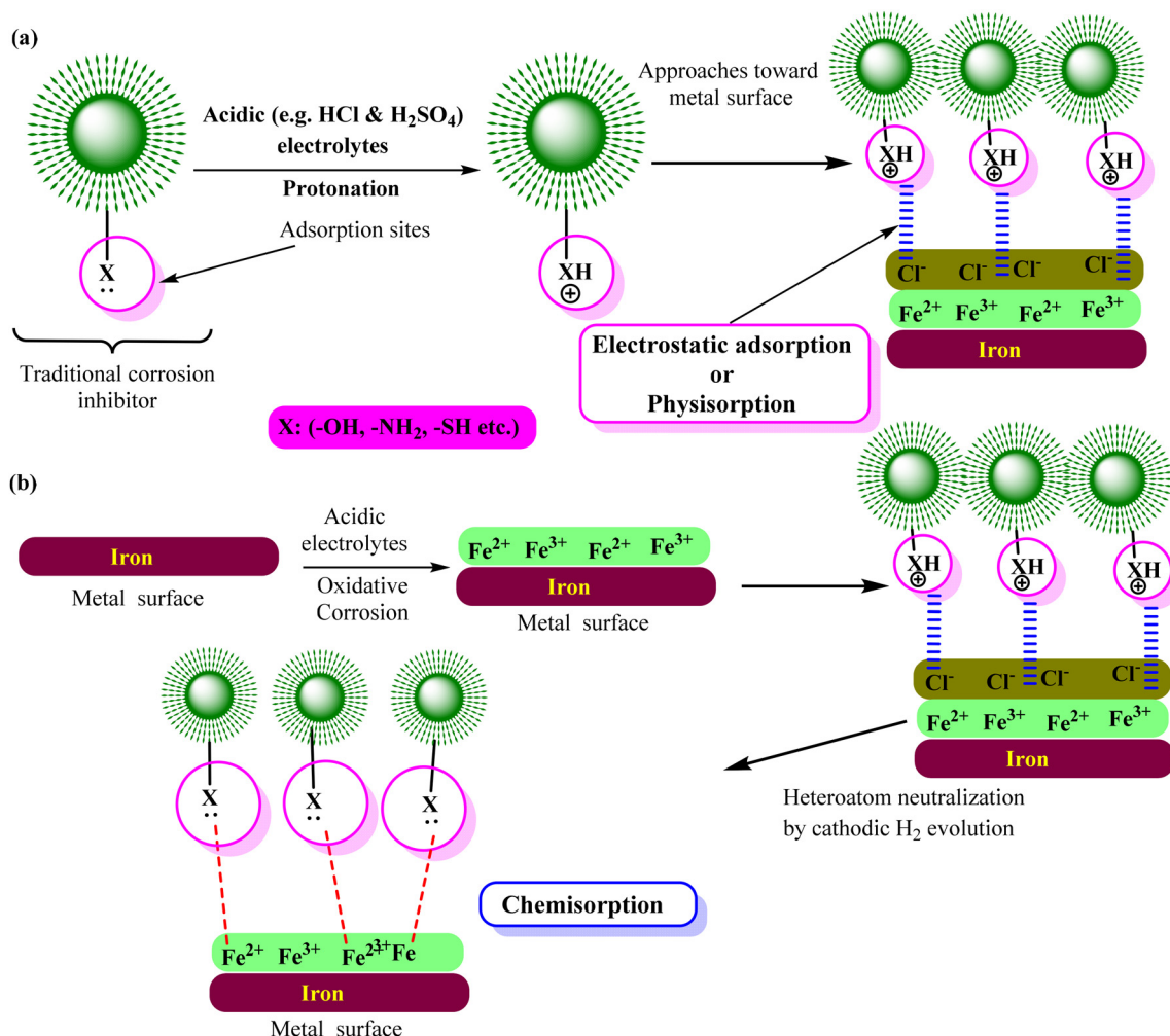
Fig. 5 Schematic presentation of the adsorption of a corrosion inhibitor having an amino ( -\text{NH}_2 ) substituent on steel surface in acidic ( \text{HCl} , \text{H}_2\text{SO}_4 , etc.) and the mode of physisorption and chemisorption [self-illustration, copyright permission not required].
