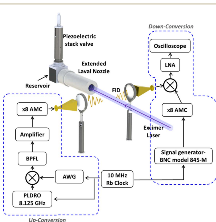
Fig. 1 Schematic illustration of the main components of the CUF experiment.
