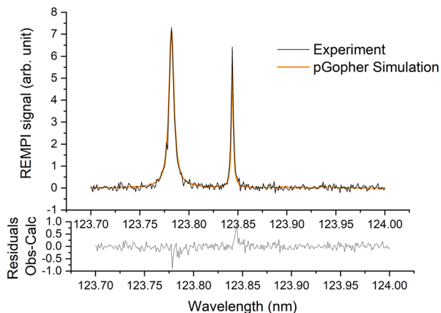
Fig. 2 Experimental (in black) and simulated (in orange) (2 + 1) REMPI spectra of the C^1B_1, v' = 0 \leftarrow X^2A_1, v = 0 transition of HDO in the supersonic beam. See Yang et al. 21 for more details.
