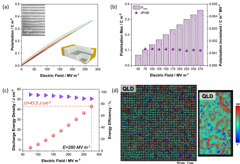
Fig. 14 QLD type MLCCs performance. (a) Unipolar P - E curves of \text{NNTa}_{0.10}\text{-10ST-2LMT} MLCCs up to the maximum field. (b) Polarisation maximum and increment as a function of electric field up to 280 \text{ MV m}^{-1} . (c) Energy storage performance up to the maximum field. (d) The [001]-oriented atomic resolution HADDF-STEM images for \text{NNTa}_{0.10}\text{-10ST-2LMT} (QLD) with the projected polarisation angle. Individual arrows show B-site cation displacement vectors in individual unit cells with different vector angles. 18 Reprinted with permission from ref. 18, the John Wiley and Sons., under the terms of the Creative Commons CC BY license.
