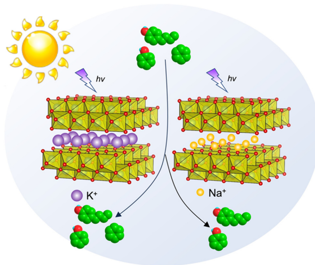
Fig. 32 Schematic of molecular recognition photocatalytic reaction induced by \text{Na}^+ -type lepidocrocite-type layered titanate with reduced layer charge density. 519
