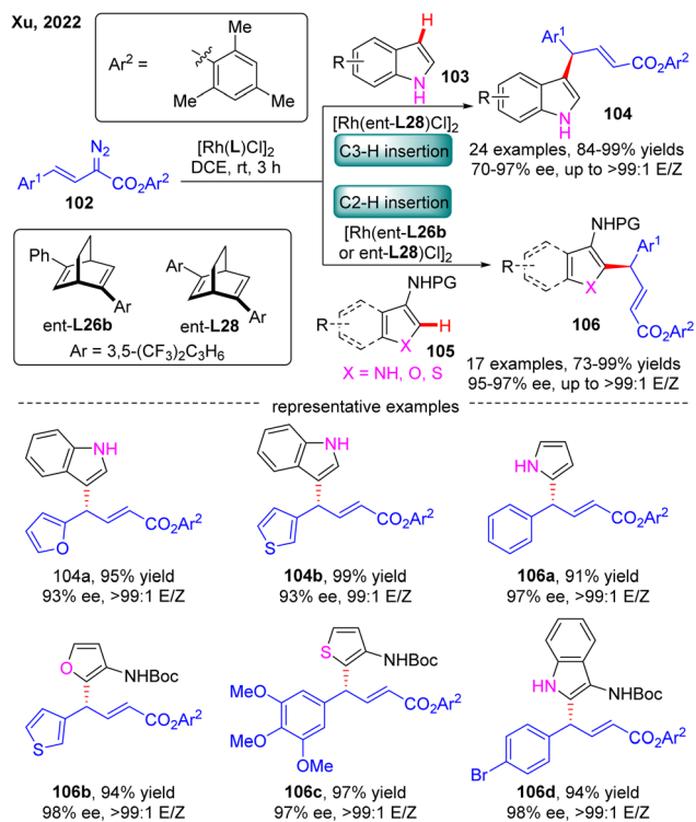
Scheme 30 Rh(i)-Catalyzed enantioselective \text{C}(\text{sp}^3)\text{-H} functionalization of 1,4-cyclohexadiene with \alpha -aryl-diazoacetates.
