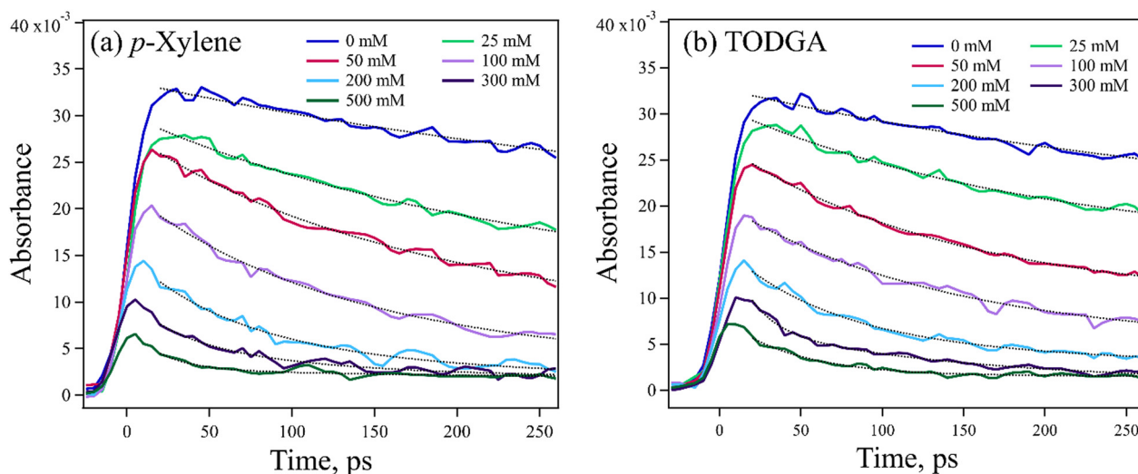
Fig. 3 Kinetic traces at 800 nm where only \text{DD}^{\bullet+} absorbs were obtained by OFSS after electron pulse irradiation, for 0–500 mM (a) p -xylene or (b) TODGA in DD with 0.3 M DCM. Dashed lines are exponential fits to the data. HT from \text{DD}^{\bullet+} to p -xylene and TODGA after pulse radiolysis are described with a sudden component ( <10 ps) followed by a resolved decay component, giving rate constants of (2.55 \pm 0.34) \times 10^{10} \text{ M}^{-1} \text{ s}^{-1} and (2.38 \pm 0.15) \times 10^{10} \text{ M}^{-1} \text{ s}^{-1} respectively.
