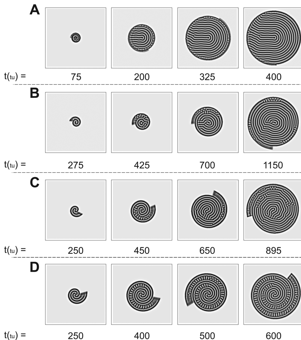
Fig. 5 Time evolution of transitional structures obtained in numerical simulations for (A) n = 0.5 ( \dot{r}_T = 0.242 \text{ su/tu} , \dot{\theta}_T = 24.0^\circ/\text{tu} ), (B) n = 1.55 ( \dot{r}_T = 8.05 \times 10^{-2} \text{ su/tu} , \dot{\theta}_T = 2.58^\circ/\text{tu} ), (C) n = 2.6 ( \dot{r}_T = 0.107 \text{ su/tu} , \dot{\theta}_T = 2.05^\circ/\text{tu} ), and (D) n = 3.6 ( \dot{r}_T = 0.161 \text{ su/tu} , \dot{\theta}_T = 2.22^\circ/\text{tu} ) in a 200 \text{ su} \times 200 \text{ su} domain.
