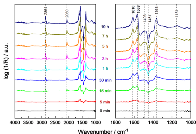
Fig. 4 DRIFT spectra during illumination of 0.1Pt/STO exposed to a constant flow of methanol (0.5%) and water (1.5%) in He (left). The spectral region 1800\text{--}1000\text{ cm}^{-1} is enlarged (right). As background spectra, the spectra before illumination at 100\text{ }^{\circ}\text{C} were chosen revealing the differences to the experiments before illumination.
