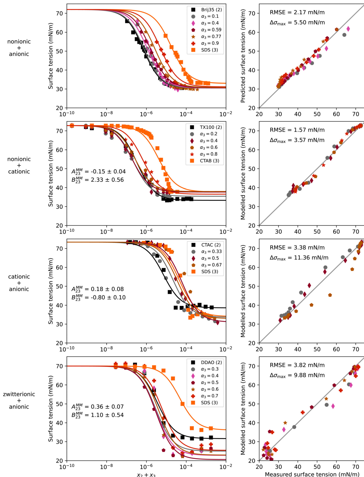
Fig. 4 Surface tension of four water-surfactant systems as a function of the solute mole fraction x_2 + x_3 . Left panels show experimental data (symbols) and model results (solid lines) from eqn (4), (8), (12), and (13). Right panels show the error in predicted surface tension for all ternary data points. The dry mole fraction \alpha_3 is defined as x_3/(x_2 + x_3) . First row: Water (1) + Brij35 (2) + SDS (3), T = 25^\circ\text{C} , data from Zakharova et al. 50 Second row: Water (1) + TX100 (2) + CTAB (3), T = 20^\circ\text{C} , data from Szymczyk and Janczuk. 51 Third row: Water (1) + CTAC (2) + SDS (3), T = 24^\circ\text{C} , data from El Haber et al. 40 Fourth row: Water (1) + DDAO (2) + SDS (3), T = 25^\circ\text{C} , data from Tyagi et al. 41 Binary fits are shown in Fig. S7 in the ESI.†
