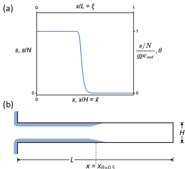
Fig. 1 (a) The representative saturation profile as a function of the distance from the channel entrance. (b) The schematic geometry of the LHA channels used to simulate ALD growth inside the channel for varying Knudsen numbers.
