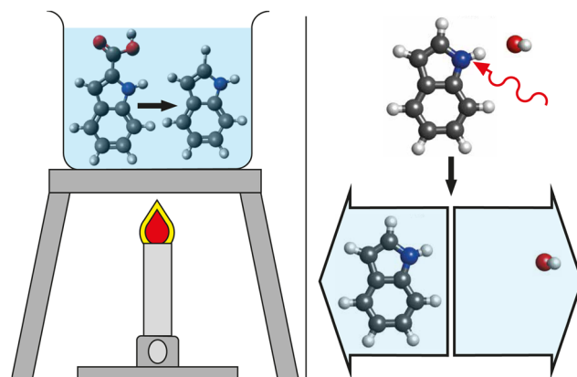
Fig. 1 Cartoon depictions of thermal-energy chemical reactions. (left) The heating by a Bunsen burner induces the final decarboxylation step of the Reissert indole synthesis in solution. (right) The mode-specific excitation of the N–H bond of a solvated indole system using a single photon of mid-IR light (red arrow) leads to bond breaking and the dissociation of the molecular system.
