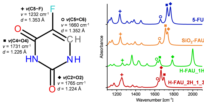
Fig. 4 Left: 5-FU molecule including bond distances and stretching frequencies of the four most prominent modes in the wavenumber range from 1200 to 1800 \text{ cm}^{-1} . Right: DFT-calculated IR spectra of free 5-FU (top curve) and adsorbed 5-FU. Spectra are normalised to have the same maximal intensity in the shown wavenumber range.
