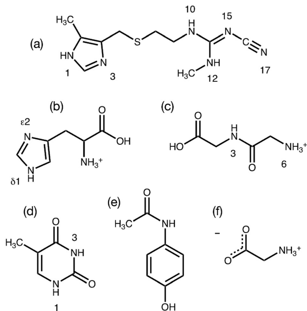
Fig. 1 Structures of the benchmark compounds studied showing nitrogen numbering. The structures evaluated include cimetine (a), histidine HCl H 2 O (b), glycylglycine HCl H 2 O (c), thymine (d), acetaminophen (e), and zwitterionic glycine (f).
