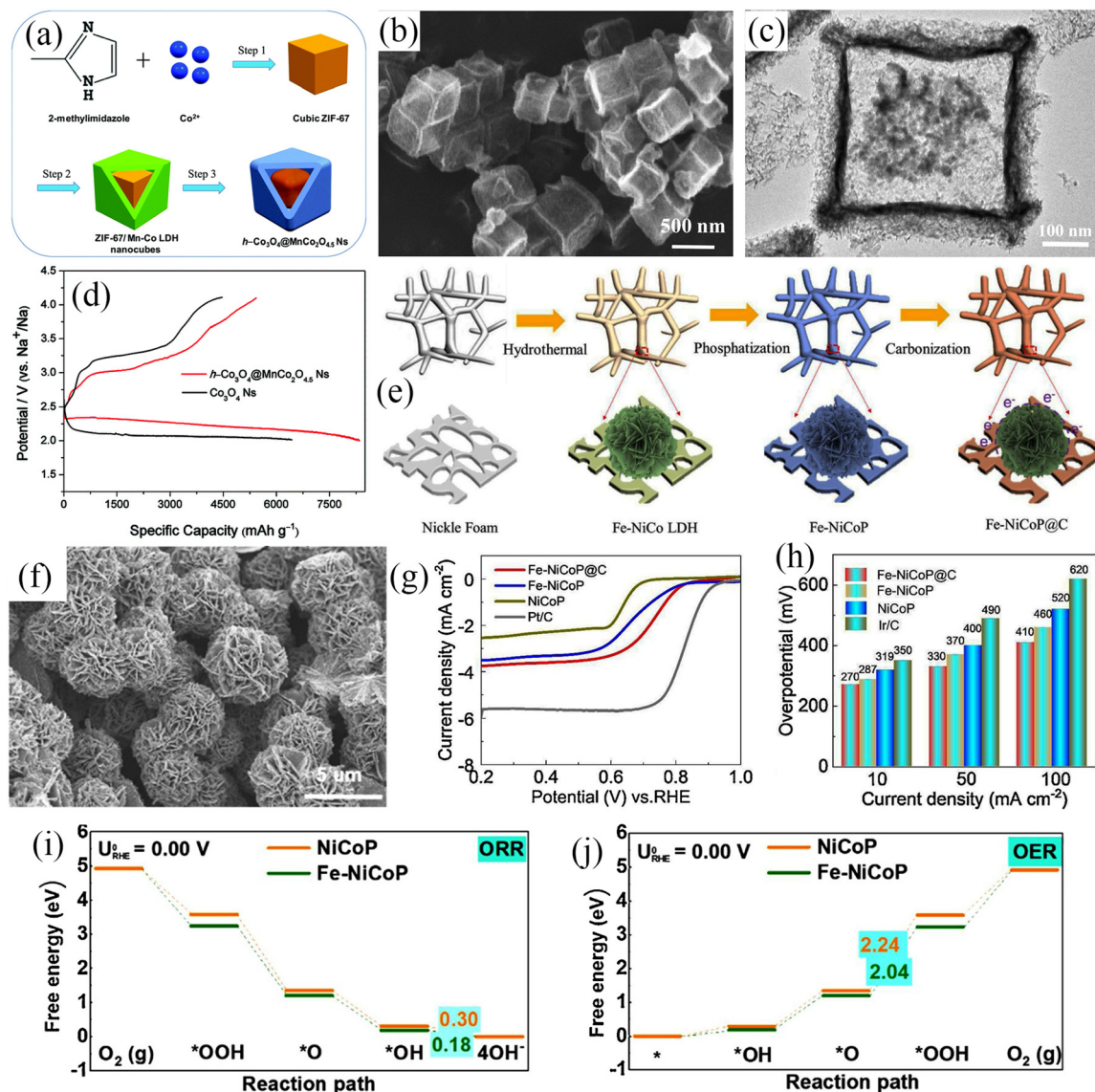
Fig. 17 (a) Scheme for the preparation of h\text{-Co}_3\text{O}_4@MnCo_2O_{4.5} Ns. (b) The SEM image and (c) The TEM image of h\text{-Co}_3\text{O}_4@MnCo_2O_{4.5} Ns. (d) The initial discharge/charge profiles of Na- O_2 batteries with h\text{-Co}_3\text{O}_4@MnCo_2O_{4.5} Ns and Co_3O_4 Ns electrodes. (Reproduced from ref. 156 with permission from the Royal Society of Chemistry). (e) Scheme for the preparation of Fe-NiCoP@C. (f) The SEM image of Fe-NiCoP@C. (g) ORR polarization curves of NiCoP, Fe-NiCoP, Fe-NiCoP@C, and Pt/C electrode. (h) The overpotentials of NiCoP, Fe-NiCoP, Fe-NiCoP@C, and Ir/C electrode. (i and j) Calculated OER/ORR energy diagram of the NiCoP and Fe-NiCoP. (Reproduced from ref. 17 with permission from the Elsevier).
