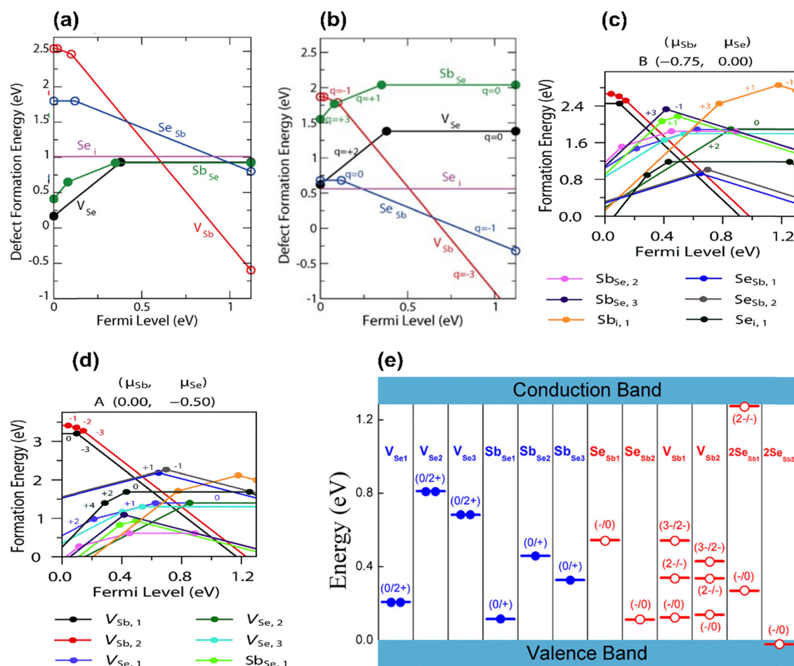
Fig. 5 The calculated formation energy of point defects in Sb_2Se_3 as a function of the Fermi level under (a) Se-rich condition and (b) Se-poor condition. 78 Defect transition-level diagrams for Sb_2Se_3 under limiting chemical potential conditions (c) Se-rich condition and (d) Se-poor condition, plotting defect formation energy (eV) against the position of the Fermi level above the VBM. 75 (e) Transition energy levels of intrinsic defects in the bandgap of Sb_2Se_3 . Red-colored levels and blue-colored levels indicate acceptor-type and donor-type defects, with their possible ionization states written above. 30
