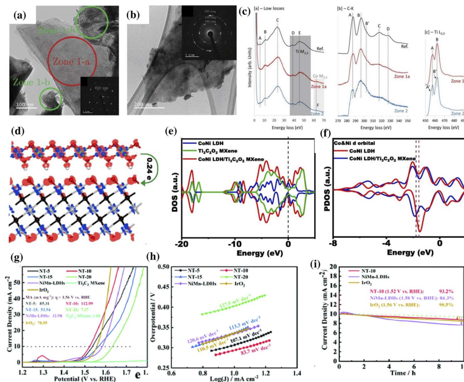
Fig. 6 TEM image depicting the (a) clean stack of Ti 3 C 2 T x sheets (Zone 1-a), fibrous Co-LDH (Zones 1-b), and (b) MXene covered with Co (Zone 2). The corresponding low loss spectra, C-K edge, and Ti L 2,3 edge recorded in Zones 1-a and 2 are shown in (c). Reproduced with permission from ref. 156 copyright 2019, Wiley. (d) Charge distribution in the CoNi LDH/Ti 3 C 2 O 2 composite, (e) DOS of CoNi LDH, Ti 3 C 2 O 2 , and CoNi LDH/Ti 3 C 2 O 2 composites with the Fermi level at zero. (f) PDOS of the Co and Ni 3d orbitals of bare CoNi LDH and CoNi LDH/Ti 3 C 2 O 2 composites. Reproduced with permission from ref. 135 copyright 2020, Elsevier. (g) Linear sweep voltammetry, (h) Tafel slope, and (i) long-term stability curves of NiMn-LDHs/Ti 3 C 2 -MXene (ref. 140).
