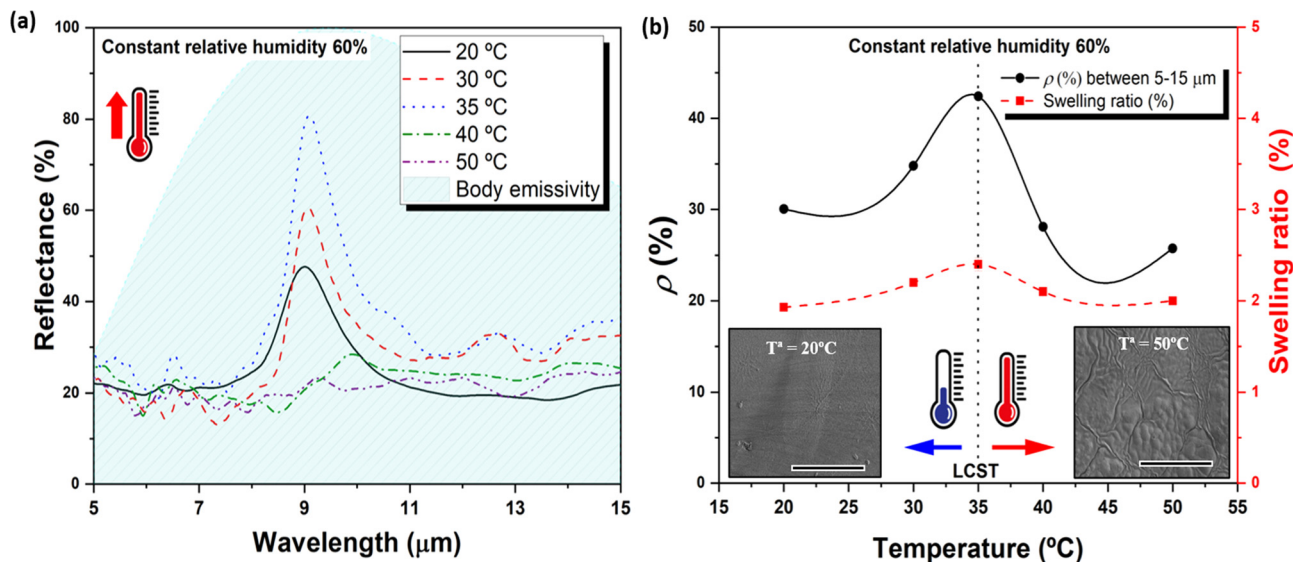
Fig. 4 (a) Evolution of the reflectance in the 5–15 \mu\text{m} range of the PNIPAM-based hydrogel composite containing 20 wt% of \text{SiO}_2 as a function of the temperature at constant relative humidity of 60%, with the human body emissivity at a skin temperature of 34 °C. (b) Percentage of infrared radiation emitted by the human body that is reflected by the PNIPAM-based hydrogel composite containing 20 wt% of \text{SiO}_2 (black circles) as well as the swelling ratio (red squares) with respect to the temperature.
