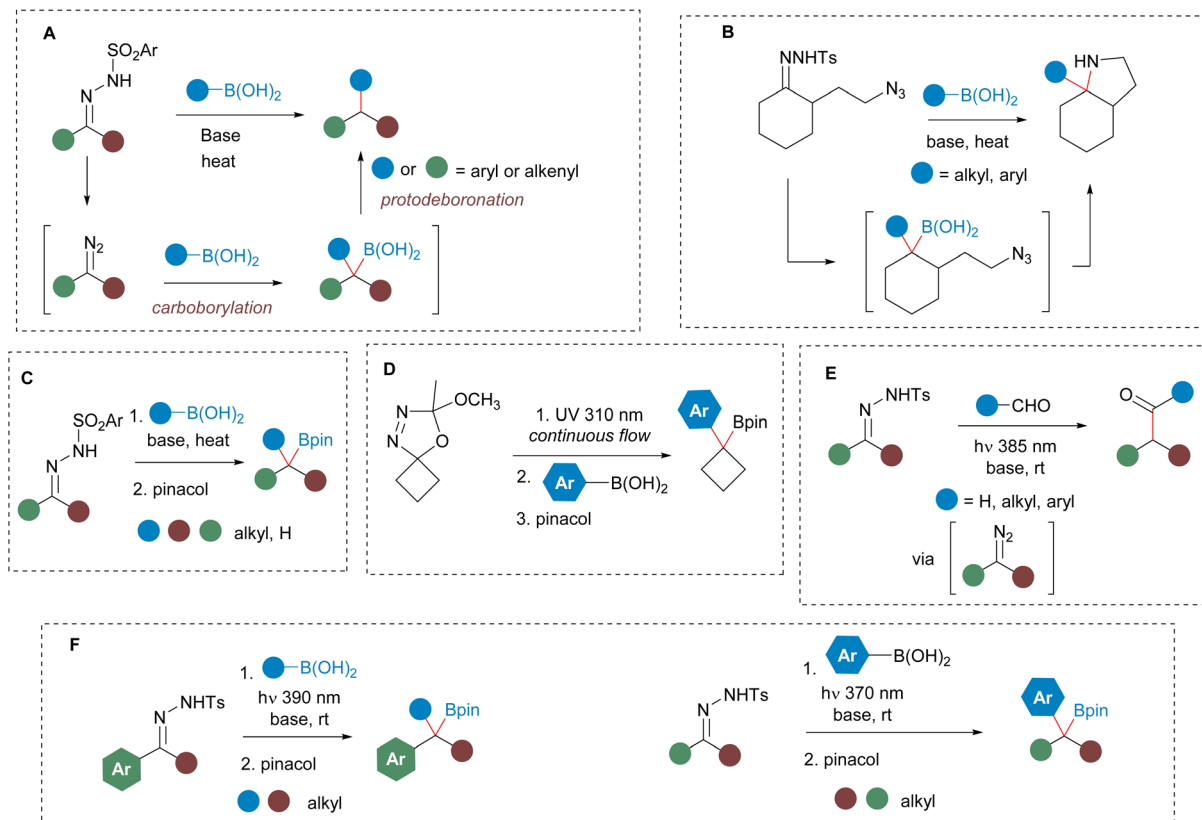
Scheme 1 (A) Reductive coupling of boronic acids and N -sulfonylhydrazones by the carboborylation/protodeboration sequence. (B) Synthesis of pyrrolidines by a C–C/C–N bond forming cascade involving carboborylation of a N -tosylhydrazone and intramolecular interception by an azide. (C) Synthesis of pinacol boronates from alkyl N -tosylhydrazones and alkylboronic acids. (D) Synthesis of benzyl boronates by photochemically promoted homologation of arylboronic acids with oxadiazolines. (E) Photoinduced generation of diazo compounds from N -tosylhydrazones and their use in the homologation of aldehydes. (F) This work: synthesis of benzyl boronates by photochemically promoted homologation of alkyl and arylboronic acids with N -sulfonylhydrazones.
