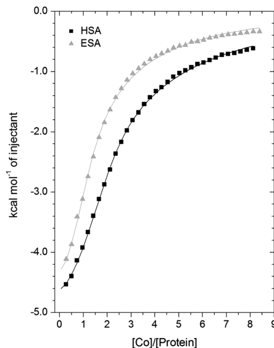
Fig. 5 Measurement of \text{Co}^{2+} binding to plasma-purified HSA and ESA using ITC. In all cases, 50\ \mu\text{M} of respective protein was titrated with 2\ \text{mM} cobalt(II) chloride solution for 35 injections. The data were fitted with a 3-sequential-sites model using MicroCal Origin 7.0 software (Fit 1–2).
