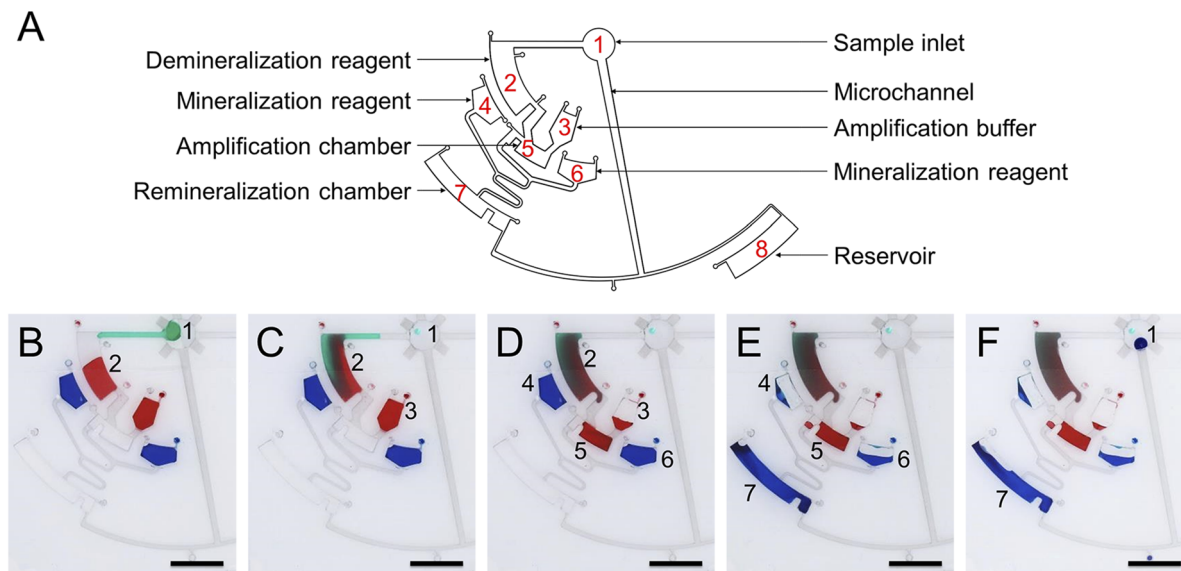
Fig. 4 Operation of the CD microfluidic chip. (A) Structure of the CD microfluidic chip and functional partitions. (B) Original state. Target DNA is mineralized with calcium carbonate nanoparticles in the original sample. (C) The sample in chamber one is driven into chamber two at 350 rpm. Mineralized target DNA is released with reagents for demineralization. (D) The demineralized sample in chamber two and amplification buffer in chamber three are driven into chamber five at 450 rpm. Free target DNA is amplified with RPA reagents. (E) The amplification product in chamber five and mineralization reagents in chambers four and six are driven into chamber seven at 550 rpm. The target DNA is remixed with reagents for mineralization. (F) The remineralized DNA sample in chamber seven is driven back to chamber one under capillary force. The scale bar is 1 cm.
