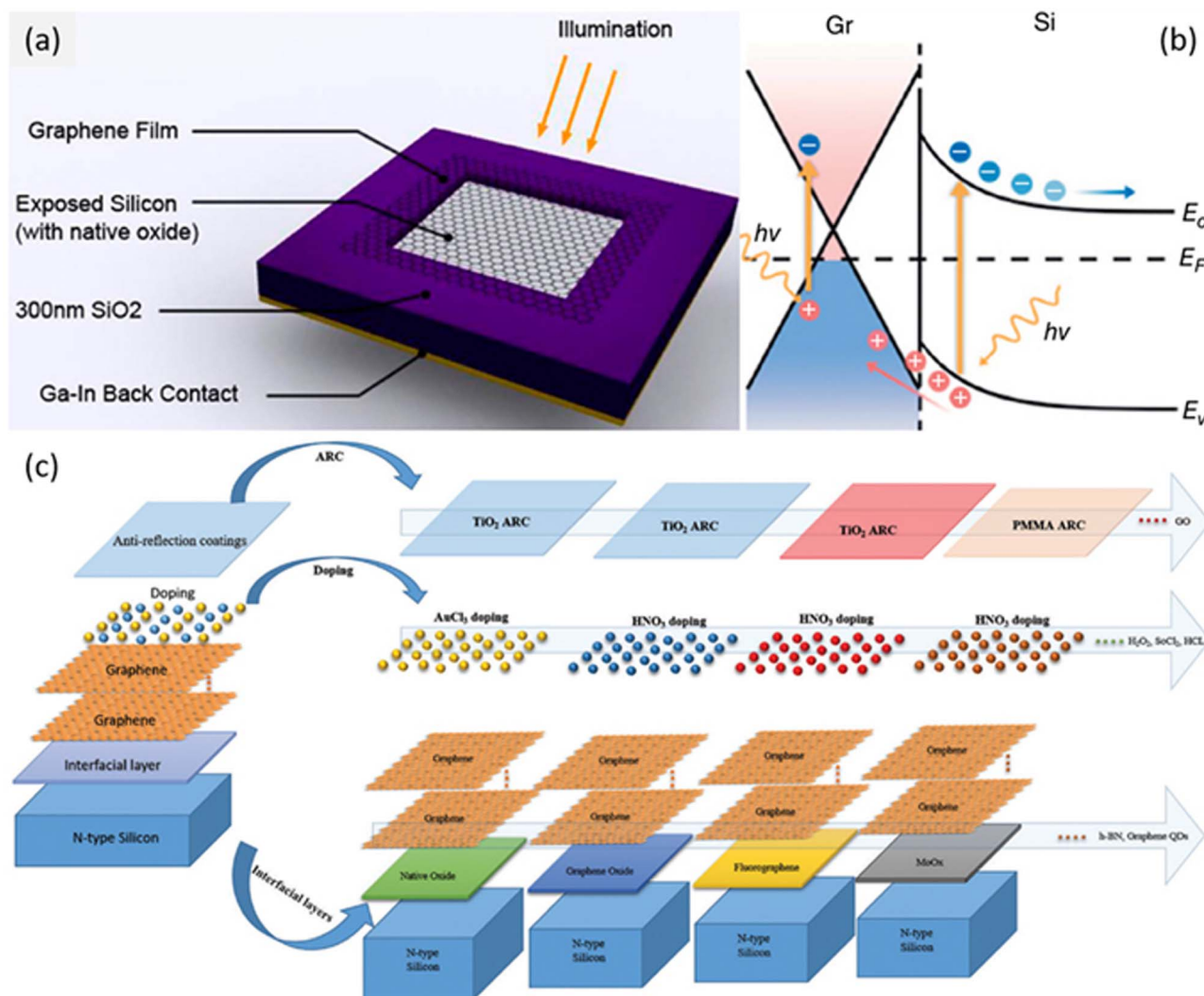
Fig. 2 (a) Design of G/n-Si SC, a layer of graphene was applied onto \text{SiO}_2/\text{Si} substrate, forming a junction. (a) has been reproduced from ref. 73 with permission from American Chemical Society. (b) Energy band diagram in G/n-Si SB-SCs and the displacement of electron-hole pairs. (b) has been reproduced from ref. 83 with permission from Wiley-VCH. (c) A visual representation depicting the uncomplicated creation of a G/Si SB-SCs through a heterojunction structure is shown. This process involves three key factors: interfacial layer, chemical doping, and ARC coating. These factors collectively contribute to improving efficiency and prolonging the durability of G/Si SCs. (c) reproduced from ref. 84 with permission from Royal Society of Chemistry.
