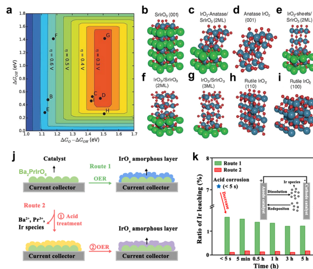
Fig. 8 (a) Theoretical overpotential volcano plot based on the scaling relation of 3C-SrIrO 3 system. (b–i) Surface models of \text{IrO}_x and 3C-SrIrO 3 , where (b–i) correspond to (b–i) in the volcano plot in (a). (a–i) Reprinted with permission from ref. 90. Copyright 2016, American Association for the Advancement of Science. (j) Schematic of two experimental routes for \text{Ba}_2\text{PrIrO}_6 in the catalytic corrosion test. (k) Comparison of the percentage of Ir leaching from \text{Ba}_2\text{PrIrO}_6 in Route 1 and 2 ratios during the OER test. (j and k) Reprinted with permission from ref. 34. Copyright 2022, Elsevier.
