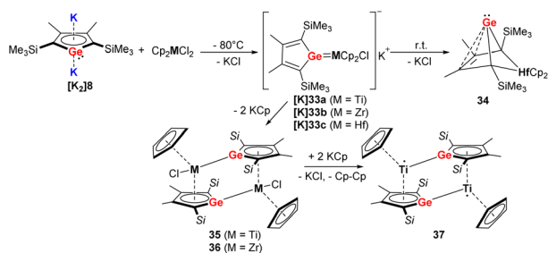
Scheme 6 Reaction of Müller's dipotassiumgermole [\text{K}_2]\text{8} towards group 4 metallocene dichlorides. 35,36
