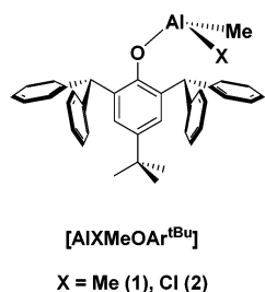
Fig. 1 Aluminium complexes used in this study.
