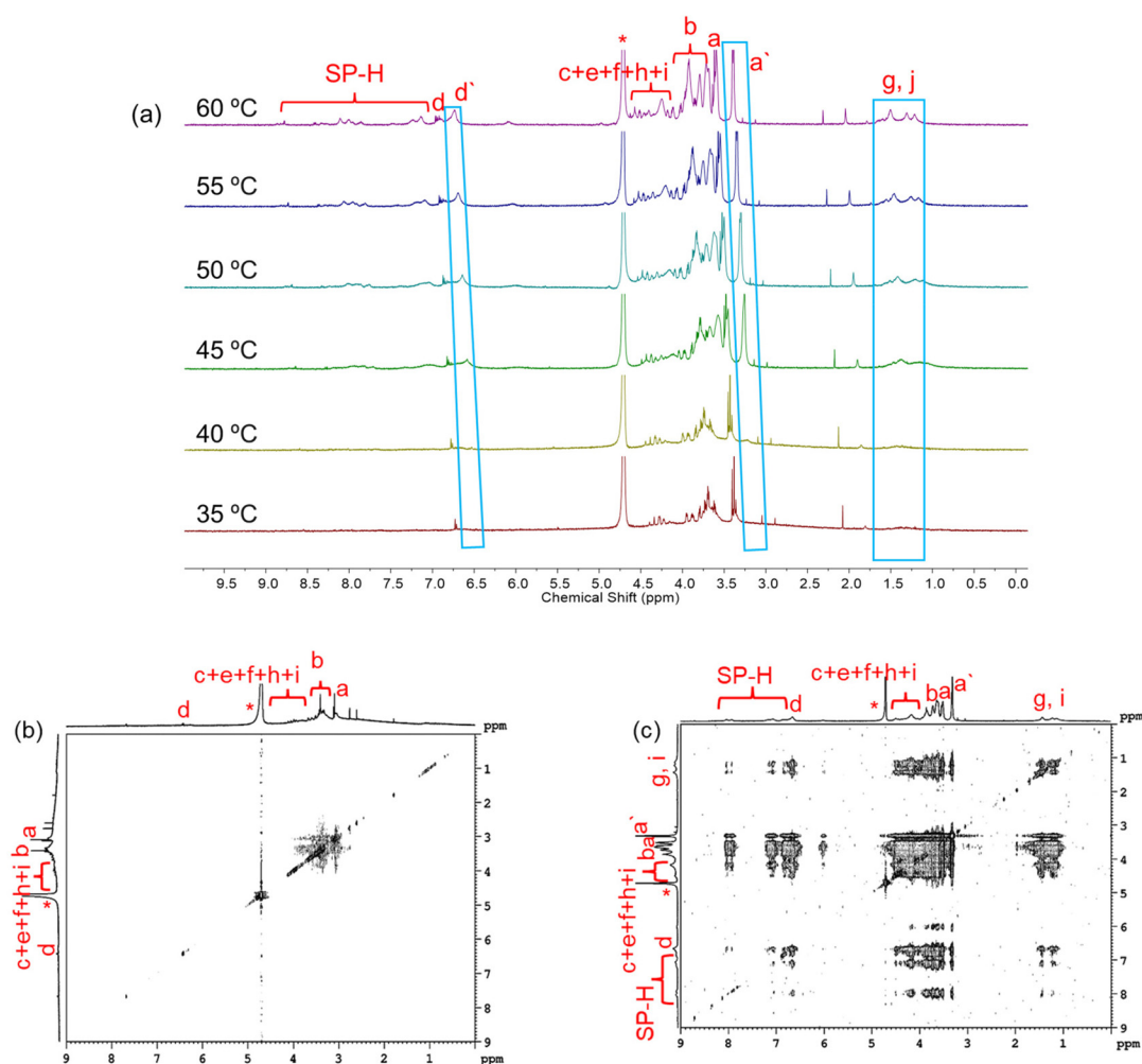
Fig. 8 1 H NMR spectra of SP-GA-MeG1 in D 2 O at varied temperatures ( C = 2.5 \text{ mg mL}^{-1} ) (a), and its NOESY spectra in D 2 O at 10 °C (below the T_{cp} ) (b) and 50 °C (above the T_{cp} ) (c) at a concentration of 5 \text{ mg mL}^{-1} .
