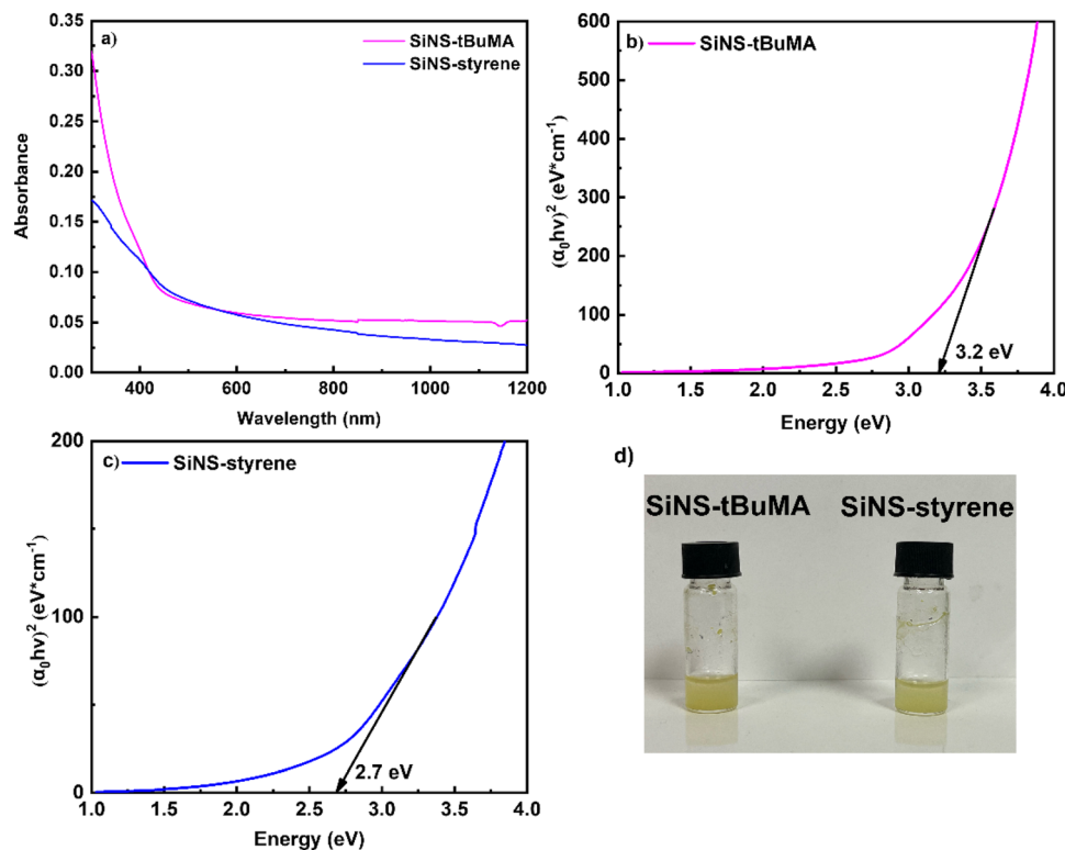
Fig. 2 (a) UV-Vis-NIR absorption spectra of SiNS- t BuMA and SiNS-styrene dispersions in toluene. Tauc plot diagrams of (b) SiNS- t BuMA and (c) SiNS-styrene for direct optical transitions. (d) Photos of SiNS- t BuMA and SiNS-styrene dispersed in toluene.
