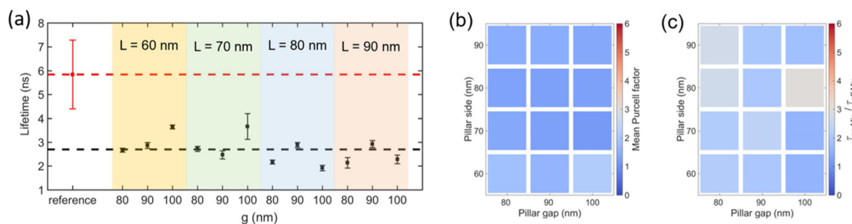
Fig. 4 (a) Measured mean luminescence lifetime of CsPbBr 3 QDs in regions with no pillars (red square) and on Mie resonators (black squares) characterized by ( L, g ) geometric parameters in the range L (60 nm–90 nm) and g (80 nm–100 nm), grouped by constant L . The selected ( L, g ) resonators correspond to those in the bottom right corner of Fig. 1, which are those indicated by a dashed line in Fig. 5. The error bars correspond to the root mean square deviations of the measured lifetimes in each region or resonator. (b) Simulated mean Purcell factor for Mie resonators characterized by ( L, g ) geometric parameters in the range L (60 nm–90 nm) and g (80 nm–100 nm). (c) Measured mean luminescence lifetime for Mie resonators characterized by ( L, g ) geometric parameters in the range L (60 nm–90 nm) and g (80 nm–100 nm), normalized by the lifetime of perovskites deposited on regions with no pillars. The scale for the averaged Purcell factors covers the values typically observed in the spatially-resolved calculations (Fig. 3(a)).
