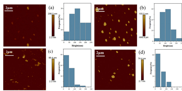
Fig. 3 AFM images and statistical size distribution of few-layer \text{NbSe}_2/\text{Nb}_2\text{O}_5 nanosheets under the centrifugation speed of (a) 1000 rpm, (b) 3000 rpm, (c) 5000 rpm, and (d) 7000 rpm.
