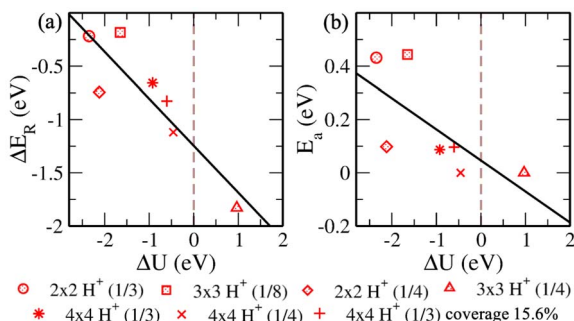
Fig. 8 (Color online) Variation of (a) reaction energy ( \Delta E_R = E_{\text{final}} - E_{\text{initial}} ) and (b) activation energy ( E_a ), of configurations with respect to the change in electrode potential ( \Delta U = U_{1_{\text{initial}}} - U_{1_{\text{final}}} ) from initial to final.
