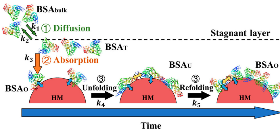
Fig. 6 A schematic representation of the adsorption process of BSA onto HM NPs. BSA molecules penetrate the stagnant layer in the vicinity of the HM NP surface ( BSA_T ) from the bulk solution ( BSA_{bulk} ) at a rate constant of k_1 . The diffusion of BSA back to the bulk solution occurs at a rate constant of k_2 . BSA molecules might overcome the energy barrier of adsorption, which depends on various factors, such as the steric and electrostatic forces between proteins and particles as well as the osmotic repulsion from a water layer on the particle surface, and bind to the surface of HM NPs without conformational changes in a transient state at a rate constant of k_3 ( BSA_O ). Then, adsorbed BSA molecules undergo conformational changes within 30–60 min at a rate constant of k_4 and change to an unfolded state ( BSA_U ). However, when the surface coverage exceeds a threshold, BSA molecules refold at a rate constant of k_5 ( BSA_O ). It is worth mentioning that the values of k_4 and k_5 depend on the protein surface coverage changing over time. Reprinted with permission from ref. 194. Copyright 2019. American Chemical Society.
