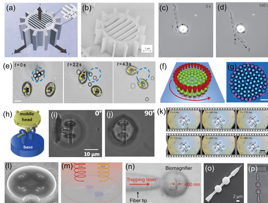
Fig. 3 OT-actuated microrobots. (a) Schematic model of birefringent microrobot. (b) Scanning electron microscopy (SEM) image of the fabricated birefringent microrobot (reproduced with permission from ref. 58. Copyright 2005, Nature Publishing Group). (c) and (d) Time-lapse images showing the use of a birefringent rotating micromotor to control the direction of growth of nerve fibers (dashed arrow) (reproduced with permission from ref. 59. Copyright 2012, Nature Publishing Group). (e) Time-lapse images showing the use of two rotating cell-based micromotors to break apart \text{SiO}_2 particle aggregate (reproduced with permission from ref. 60. Copyright 2020, American Chemical Society). (f) and (g) Schematic and microscope image of the nano-clutch. Red cones represent optical traps translating 27 microparticles on a circular path (counter-clockwise rotation) (reproduced with permission from ref. 61. Copyright 2016, Nature Publishing Group). (h) Schematic of an articulated microrobot. (i) and (j) Out-of-plane rotation of the mobile head of the articulated microrobot with respect to various angles (reproduced with permission from ref. 68. Copyright 2016, Wiley-VCH GmbH). (k) Time-lapse images showing the process of loading cargo into the microrobot (reproduced with permission from ref. 70. Copyright 2016, Nature Publishing Group). (l) SEM image of a microdrone with four nanomotors. (m) Schematic of using light beams with different wavelengths and polarization states to drive the microdrones (reproduced with permission from ref. 71. Copyright 2022, Nature Publishing Group). (n) Microscope image showing the light-actuated bio-magnifier that can image a nanopatterned letter (reproduced with permission from ref. 72. Copyright 2019, Nature Publishing Group). (o) SEM image of a surface scanning probe and (p) optical image of the probe as it scans the surface of a sample (reproduced with permission from ref. 73. Copyright 2014, Nature Publishing Group).
