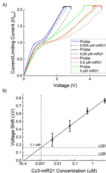
Fig. 3 Calibration of integrated AEM sensor. A) Depicts CVCs for four concentrations (0.005 \mu M, 0.05 \mu M, 0.5 \mu M, and 5 \mu M) of Cy3 labelled miR-21. For each sample a baseline (probe) CVC was measured before 4 \mu L of each concentration of Cy3 labelled miR-21 sample was loaded and concentrated ( I_{app} = 0.8 mA, V_{max} = 180 V, U = 0.12 mL h^{-1} ) for 20 minutes, flow and current were stopped and the sensor was incubated for 20 minutes before being washed with 4 \times PBS followed by 0.1 \times PBS. The I - V signal of the AEM sensor was then measured. B) The resultant voltage shifts were used to generate a calibration curve relating AEM voltage shift ( \Delta V ) to Cy3 labelled miR-21 concentration. The error bars show uncertainty at 95% with three replicants for each point, and the solid line shows a linear curve fit reflecting the log-linear behaviour of the AEM sensor. The sensor shows a dynamic range of 3 decades with a limit of detection of 1.1 nM.
