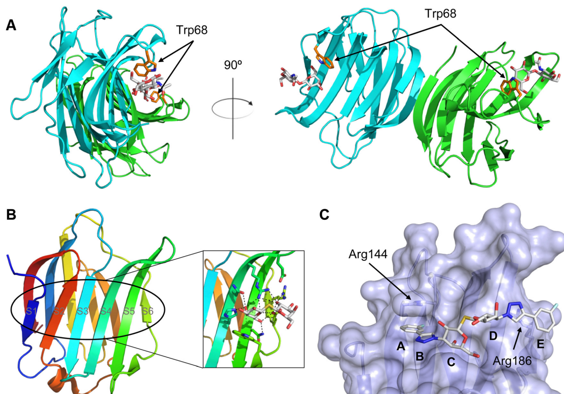
Fig. 9 Galectin-1 and -3. (A) Gal-1 in complex with LacNAc (PDB code 4XBL). 244 The essential tryptophan of the carbohydrate binding site is shown as stick. (B) Gal-3 CRD in complex with a thiodigalactoside (PDB code 4JC1) (see lit. 245 ). (C) Complex of Gal-3 with TD139 ( 55 , PDB code 5H9P). While the carbohydrate core of TD139 interacts with the subsite C and D as seen for native sugar ligands, the hydrophobic substituents interact favourably with neighbouring subsites, increasing affinity and specificity.
