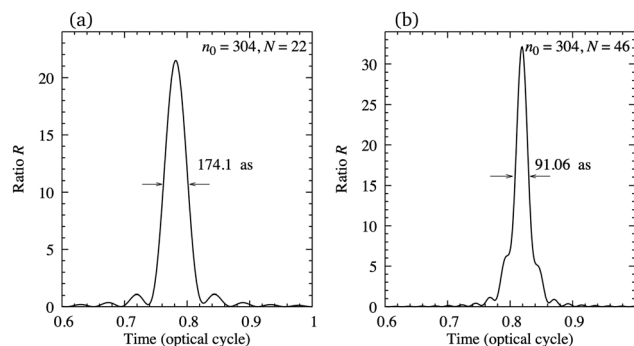
Fig. 11 Ratio R as a function of time for N = 22 [panel (a)] and N = 46 [panel (b)] harmonics, starting from n_0 = 304 , generated by exposing the \text{N}_2^+ cation to the \omega-2\omega OTC field with the same parameters as in Fig. 7.
