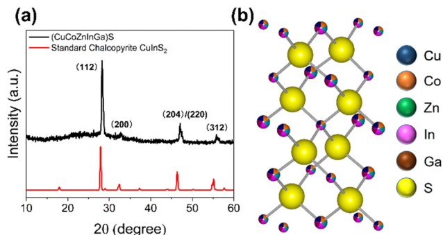
Fig. 1 Figure of (a) powder X-ray diffraction pattern of thin film (CoCuZnGaIn)S with reference to standard chalcopyrite (CuInS 2 , ICSD: 66865). (b) The crystal structure of HE chalcopyrite ( a = b = 5.52 , c = 11.13 , \alpha = \beta = \gamma = 90^\circ ).
