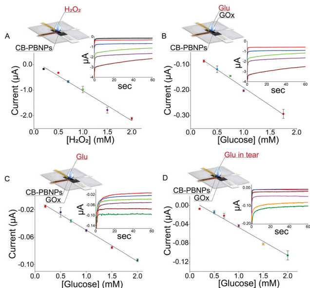
Fig. 2 (A) Calibration curve of H 2 O 2 obtained by using the paper card-like PVC device modified with CB-PBNPs. (B) Calibration curve of glucose in PBS obtained by using the paper card-like PVC device modified with CB-PBNPs. (C) Calibration curve of glucose in PBS obtained by using the paper card-like PVC device modified with CB-PBNPs and the GOx enzyme. (D) Calibration curve of glucose in artificial tears obtained by using the paper card-like PVC device modified with CB-PBNPs and the GOx enzyme. Insets: Corresponding chronoamperometric measurements.
