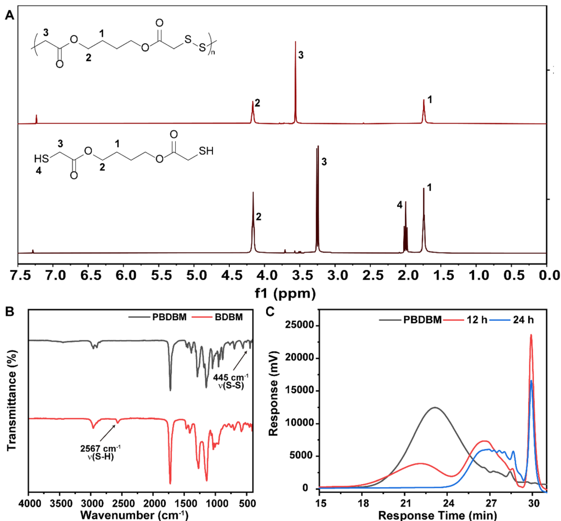
Fig. 1 Characterization of poly(disulfide)s (PBDBM). (A) 1 H NMR spectra of PBDBM and BDBM. (B) FT-IR spectra of PBDBM and BDBM. (C) GPC profiles of PBDBM and PBDBM after incubation with dithiothreitol for 12 and 24 h.
