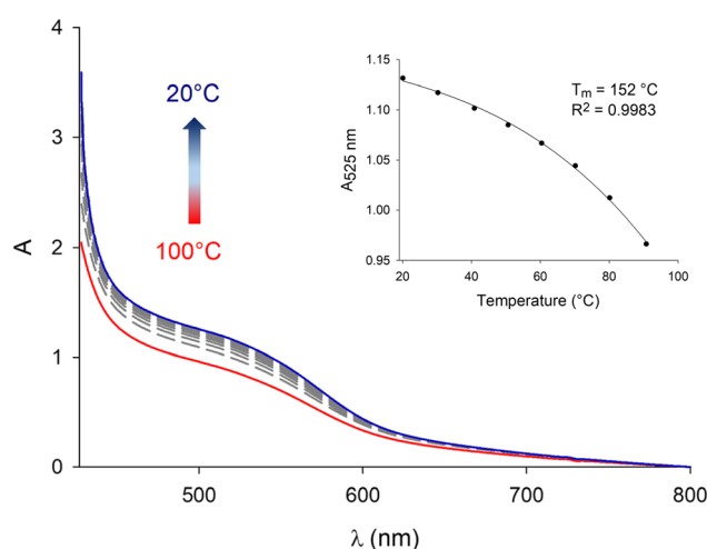
Fig. 5 Evolution of the visible absorption spectrum of a C_3 Pyr/ C_3 NDI (1:1) mixture in TCE ( [C_3\text{Pyr}] = [C_3\text{NDI}] = 5.2 \text{ mM} ) upon decreasing the temperature from 100 °C (red curve) to 20 °C (blue curve) (interval of 10 °C between each curve). Inset. Corresponding evolution of the absorbance at \lambda = 525 \text{ nm} .
