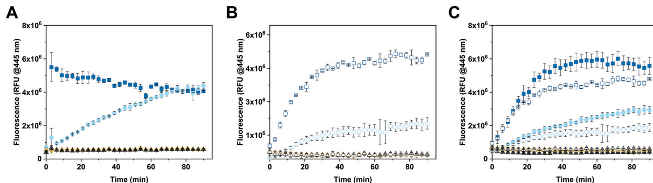
Fig. 3 Enzymatic efficiency of CNCs at 37 °C. (A) 4-MUG (5 \mu\text{M} ) conversion to 4-MU in PBS, (B) in cell culture medium supplemented with 10% fetal bovine serum (FBS), and (C) in PBS (filled symbols) and cell culture medium (empty symbols), each supplemented with 10% FBS. Squares represent free GUS (24 U \text{mL}^{-1} ), circles: GUS–melCNCs, rhombi: GUS–CNCs triangles: corresponding reaction mix without enzyme. Measurements represent triplicates, symbols might overlap.
