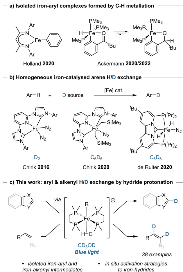
Scheme 1 a) Previous examples of isolated iron-aryl complexes by direct C–H metallation. b) Previous homogeneous iron-catalysed H/D exchange catalysts. c) This work: arene and alkene C–H metallation and H/D exchange using CD 3 OD and a bench-stable iron(II) pre-catalyst.
