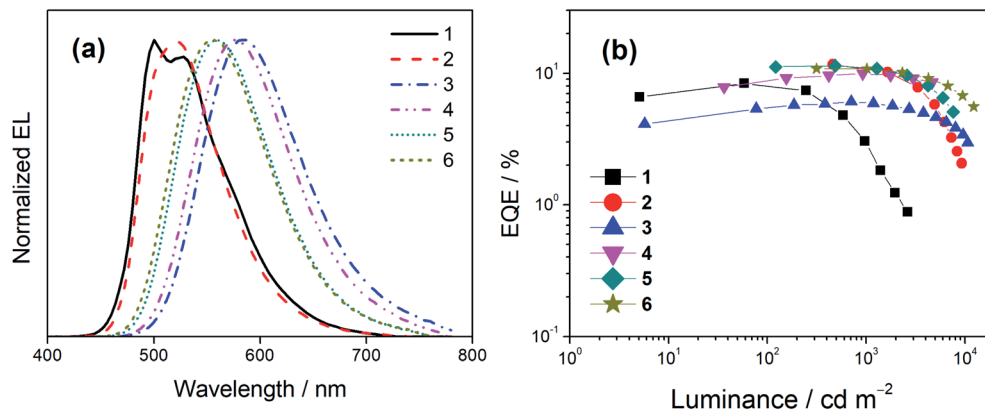
Fig. 7 (a) Normalized EL spectra and (b) EQEs of the solution-processed devices based on 1–6.
