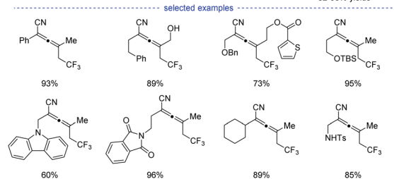
Scheme 1 Cu-catalyzed regioselective trifluoromethylcyanation of 1,3-enynes.
