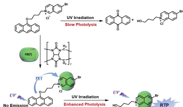
Fig. 7 Schematic illustration of construction of photoresponsive RTP supramolecular assembly by CB[7] and amphiphilic 6-bromoisoquinoline.
