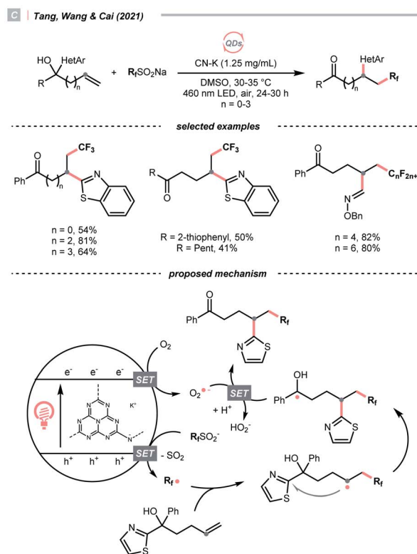
Scheme 41 R* from sulfoniums, thiazoliniums, sulfinates and sulfinamides.
