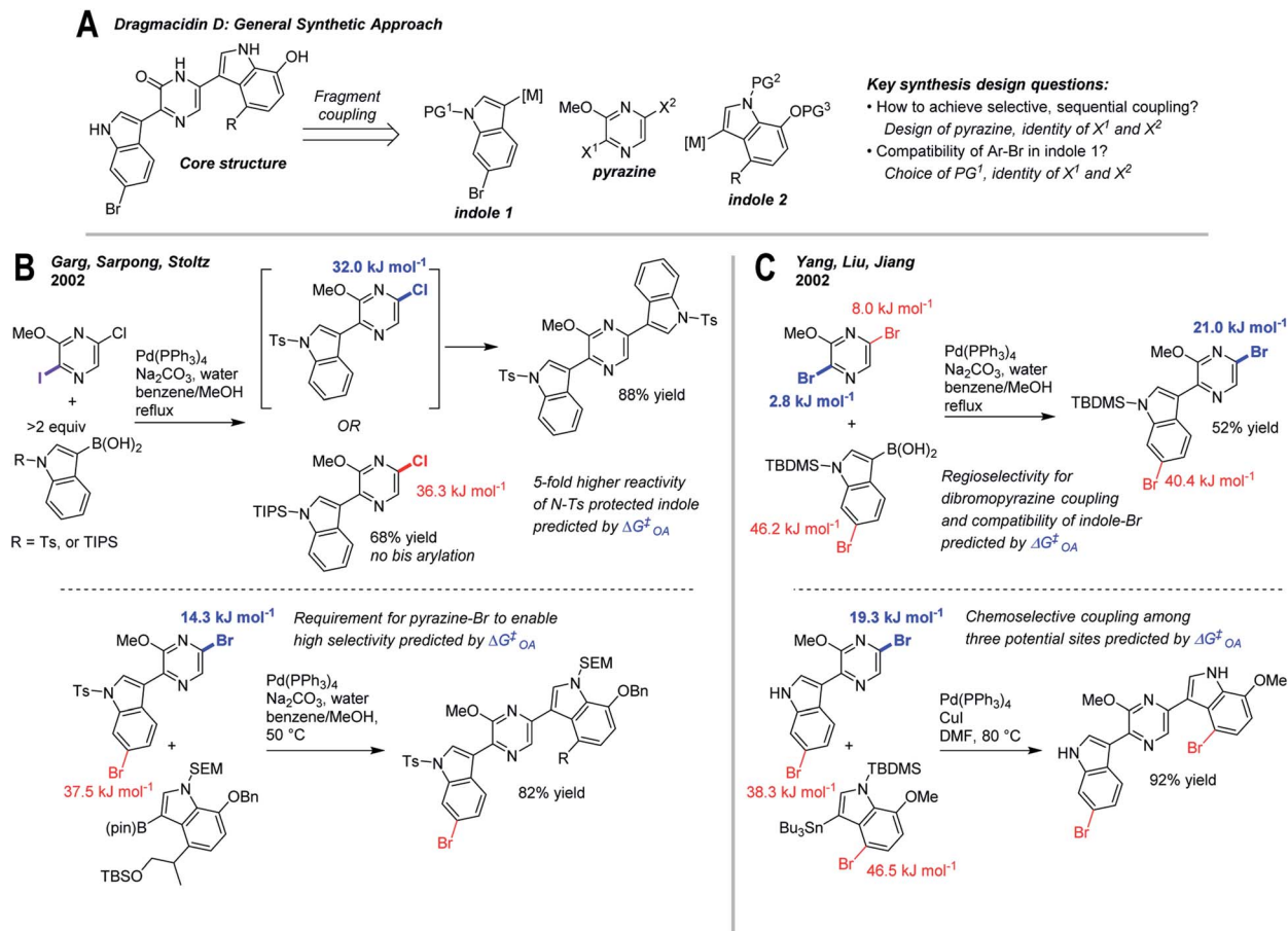
Fig. 7 Retrospective analysis of applying \Delta G_{\text{OA}}^{\ddagger} predictions to synthesis design: dragmacidin D. (A) Retrosynthesis of core structure, involving selective fragment coupling to a dihalogenated pyrazine. (B) Approach involving differential halogenation, tosylate protecting group on indole 1, and switch from 5-chloro to 5-bromopyrazine intermediates for selective coupling. 81 (C) Approach involving regioselective coupling to dibromopyrazine, TBS protecting group on indole 1, and regioselective Stille coupling. 82
