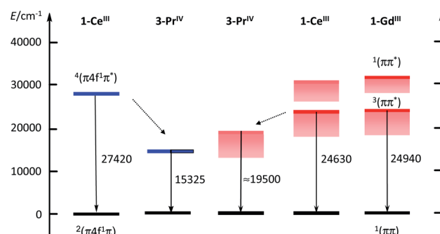
Fig. 6 Partial electronic diagram for 1\text{-Ce} , 3\text{-Pr}^{\text{MeCN}} and 1\text{-Gd} . Calculated levels in blue, experimental 0-phonon levels in red or rose when estimated from the onset of the emission band. Energies of the transitions in \text{cm}^{-1} .
